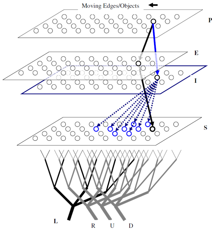
Figure 1. A schematic illustration of a direction selective neuron L and its presynaptic neural network with the left side lateral inhibition. There are four groups of cells and one single cell in the system: photoreceptor cells ( P ); excitatory and inhibitory cells ( E and I ); summing cells ( S ); the left inhibited direction selective cell L . The lateral inhibition is indicated with dotted lines between I and S layer; the excitation is indicated with black lines between E and S layer. The connections between cells in P and E , P and I , E and S are one-to-one; only the connections to example cells are illustrated in this plot. The other direction selective cells, such as R , U and D , are with different inhibition preferences.
