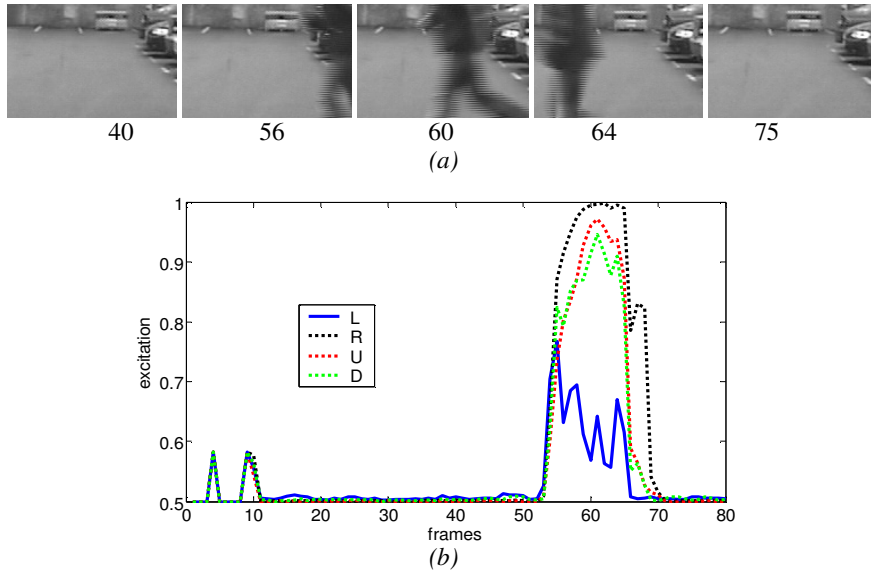
Figure 2. An example of Directional selective neurons process video sequences with a left running pedestrian. (a), sample images of the video sequences; the frame number is indicated under each image. (b), the excitation of the four Directional selective neurons: L (left), R (right), U (up) and D (down); note the left inhibited cell L 's excitation is significantly lower than the other three Directional selective neurons'.
